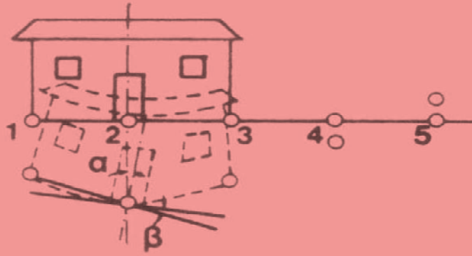
Tilt and Angular Distortion
